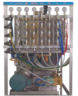
LOW PRESSURE MANIFOLDS
